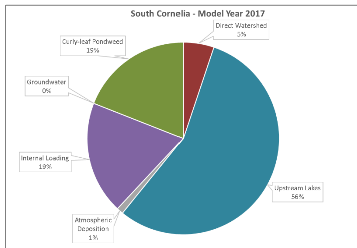
Figure 6-13 Loading Summaries from South Cornelia In-Lake Calibration Models
