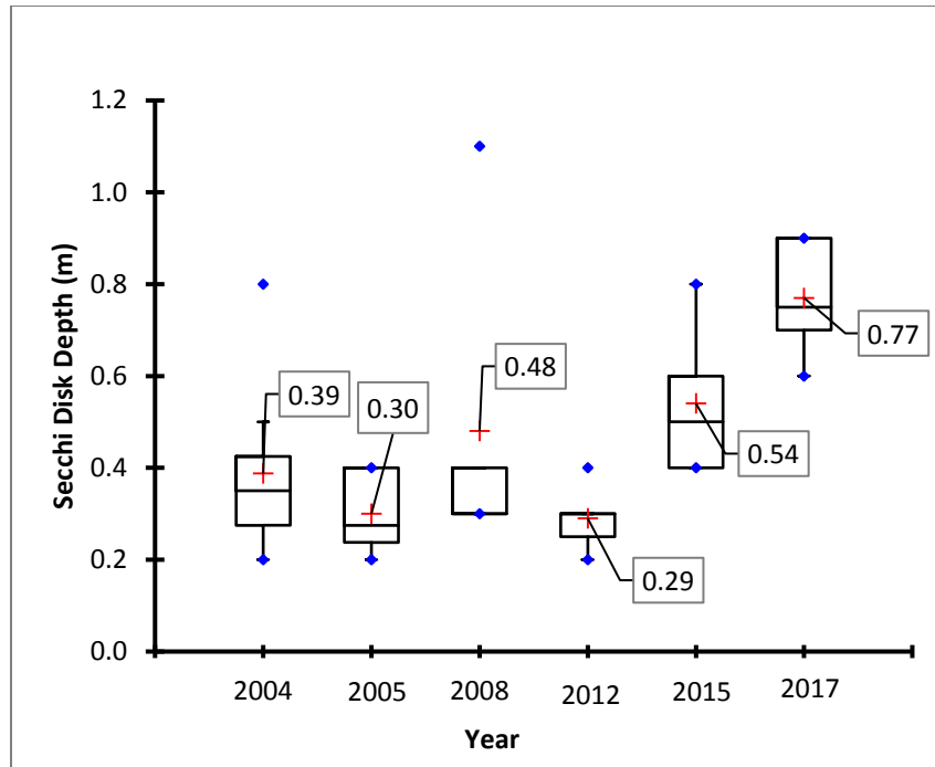
Figure 5-5 Summer Secchi disc depth readings in Lake Edina from 2004 through 2017. The red crosses indicate the average of summer (June through September) readings.
