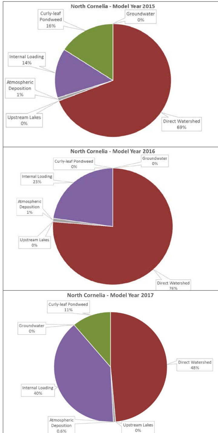
Figure 6-12 Loading Summaries from North Cornelia In-Lake Calibration Models
