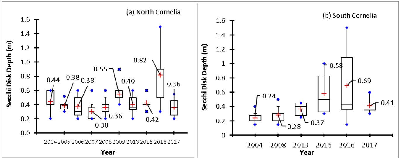
Figure 5-3 Summer Secchi disc depth readings in (a) North and (b) South Cornelia from 2004 through 2017. The red crosses indicate the average of summer (June through September) readings.
