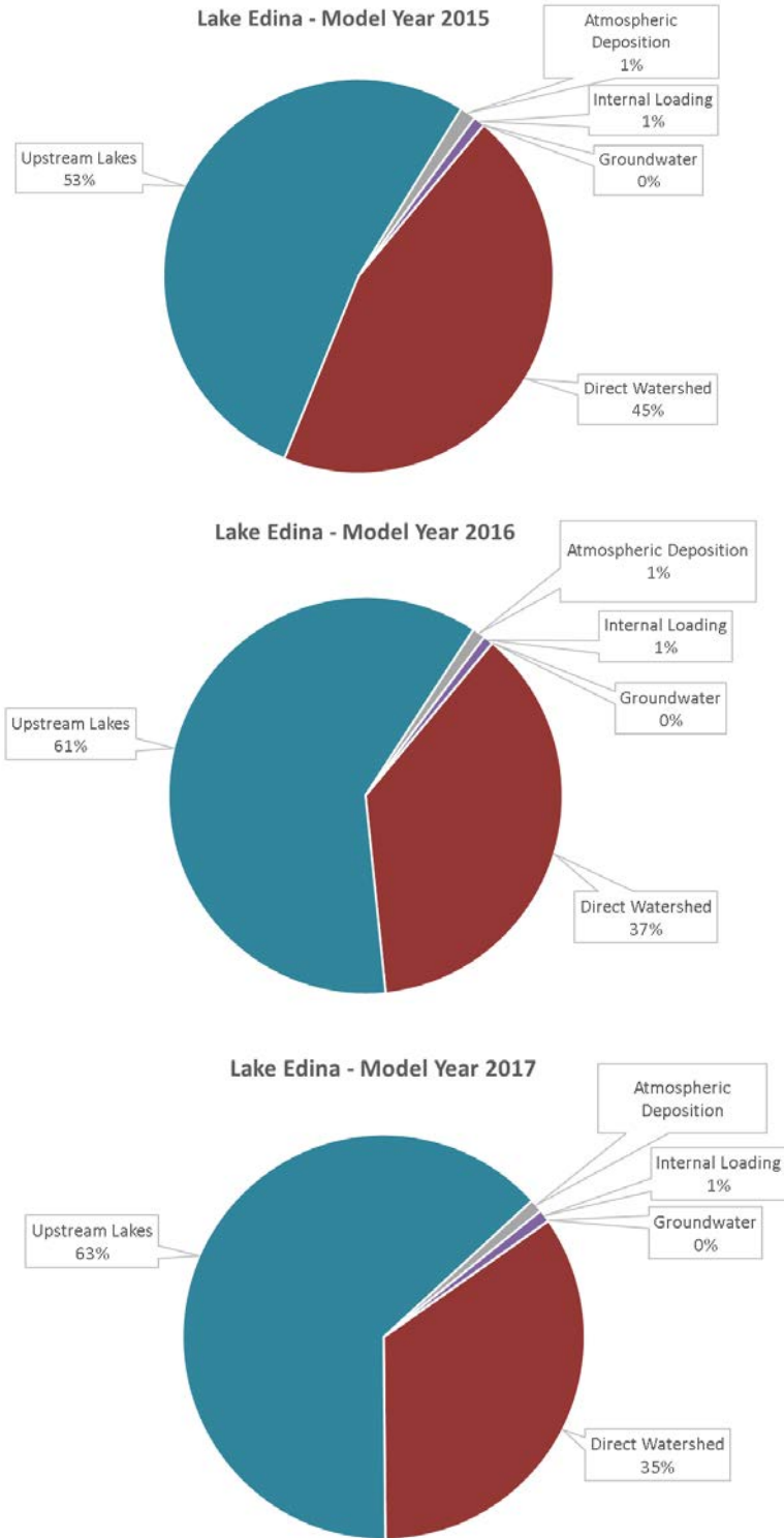
Figure 6-14 Loading Summaries from Lake Edina In-Lake Calibration Models
