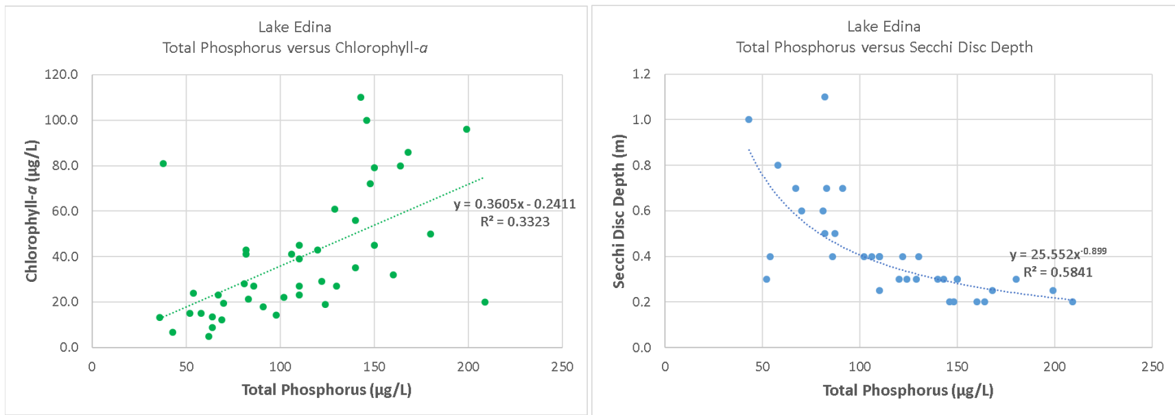
Figure 6-17 Lake Edina relationships between total phosphorus, chlorophyll a, and Secchi Disc Transparency
